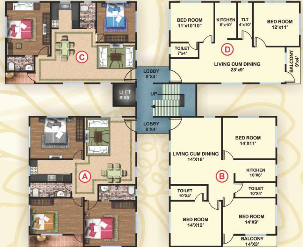
Typical Floor Plan of 3 & 2 BHK Type
